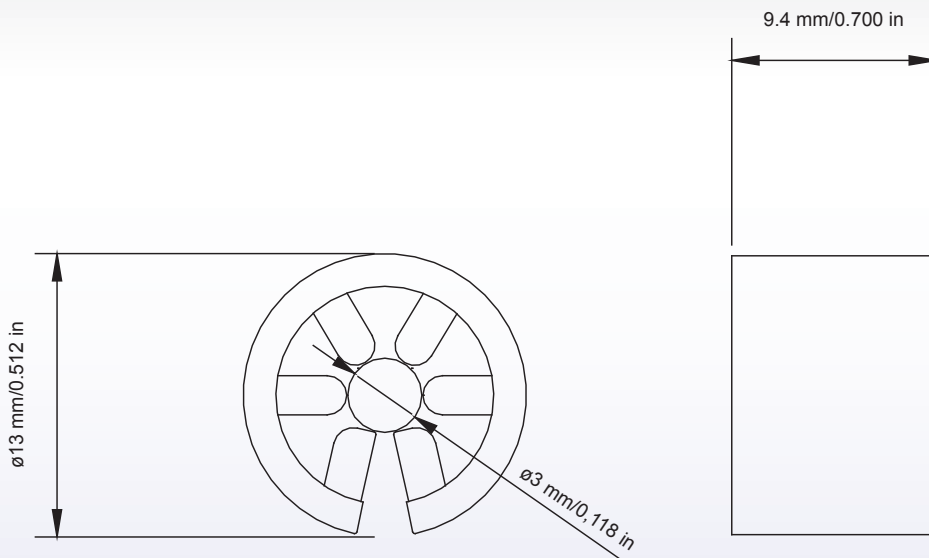
The Mini Recyclable shown from top and side. (Measurements in millimeters/inches).
