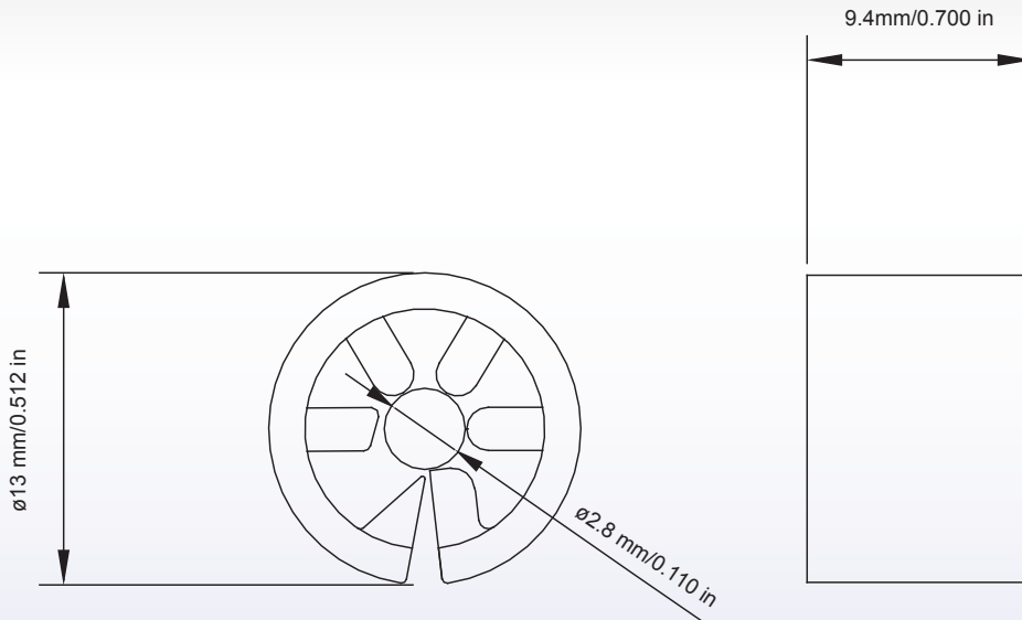
The Mini Secure shown from top and side. (Measurements in millimeters/inches).
